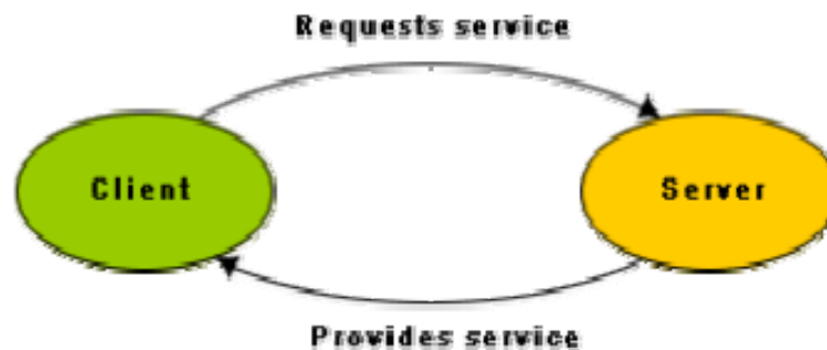
Fig. 17.1: Client-server model
